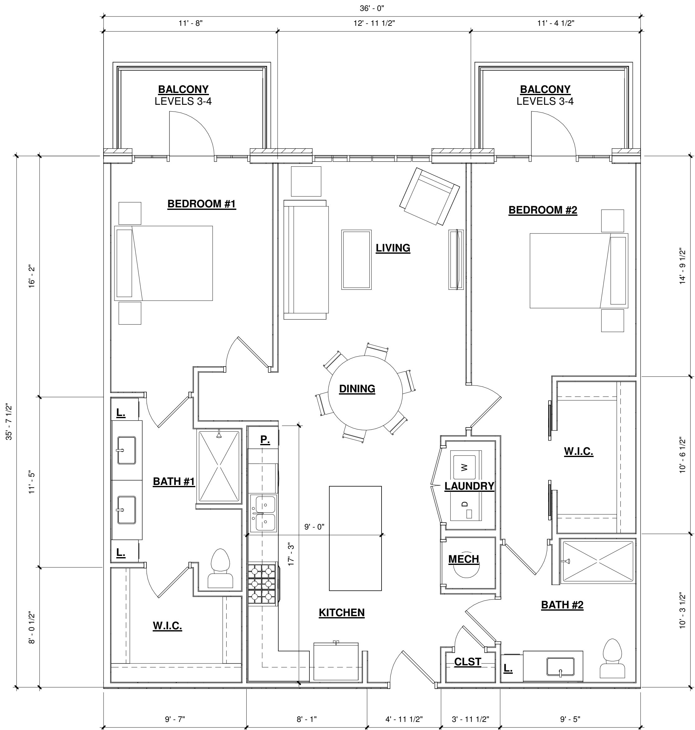
1 UNIT - B4 1/4" = 1'-0"
